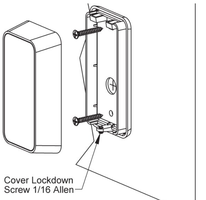
Fig. 2: BAPI-Stat "Quantum Slim" Mounting
