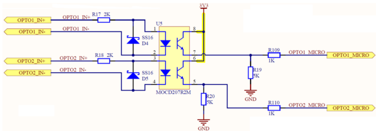
Illustration 14 : Schematics of optocouplers inputs
