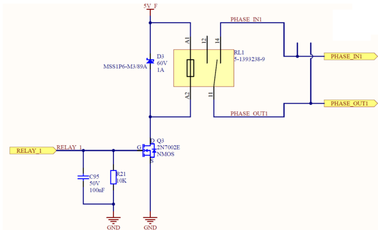
Illustration 15 : Schematics of relays outputs
