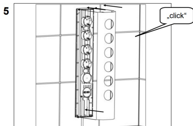
Mounting in a corner
