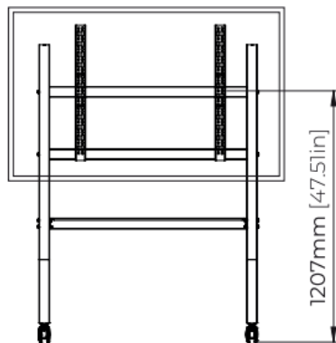
Min. Screen Height Assembly
