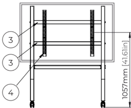
Min. Screen Height Assembly
