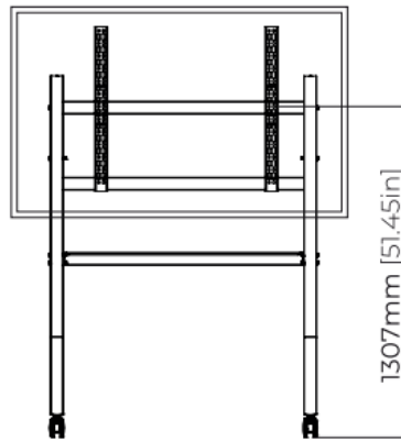
Middle Screen Height Assembly
