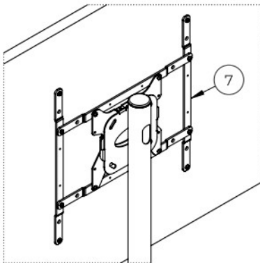
VESA 400 x 400mm installation
