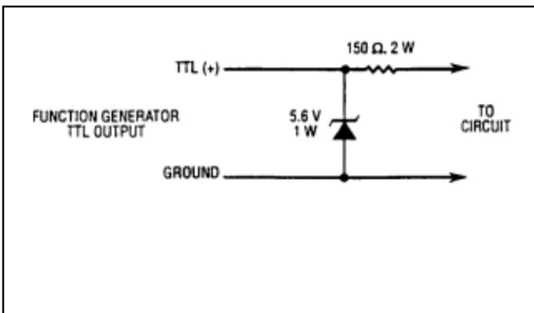
Figure 5. Circuit for Protection of TTL Output.
