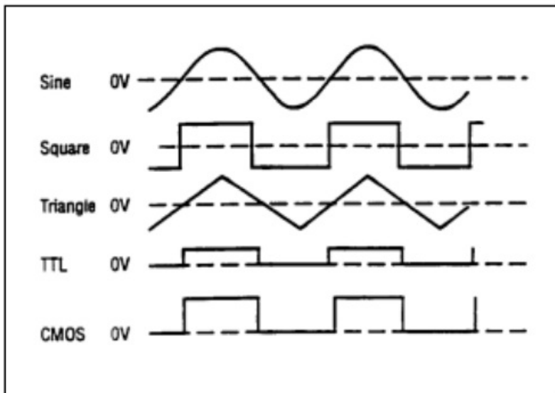
Figure 2. Output Waveform and Phase Relationship
