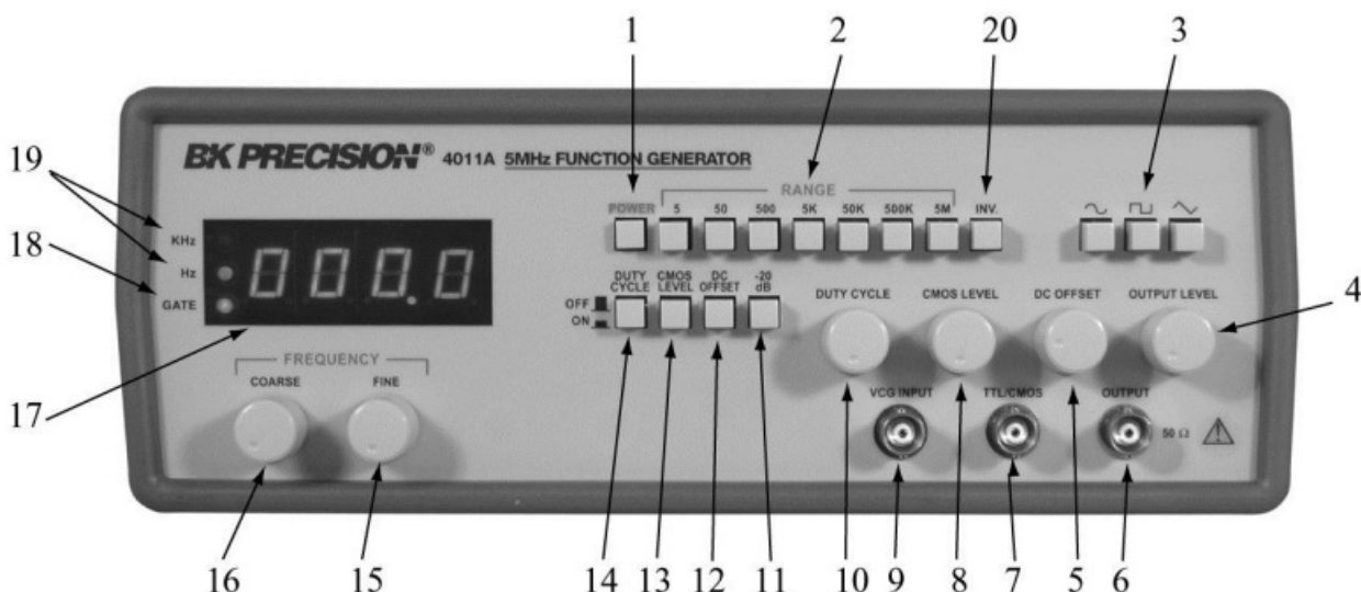
Figure 1. Model 4011A Controls and Indicators.
