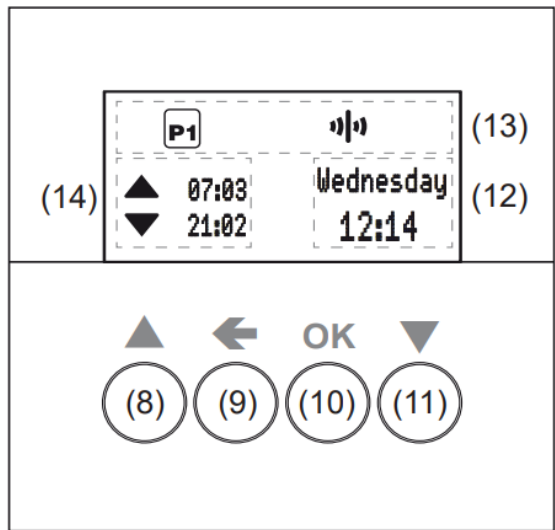
Figure 2: Display and operating elements
