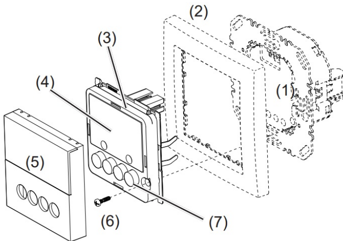
Figure 1: Design of the device
