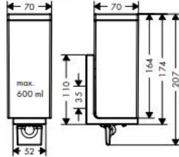
AXOR Universal Rectangular 42610XXX
