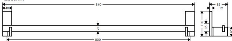
AXOR Universal Rectangular 800 42683XXX
