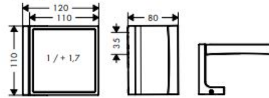
AXOR Universal Rectangular 42649XXX
