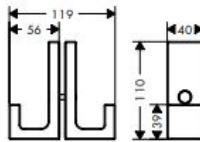
AXOR Universal Rectangular 42639XXX
