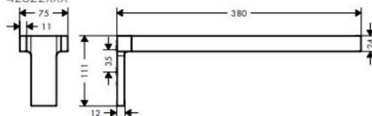
AXOR Universal Rectangular 42622XXX
