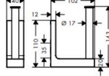
AXOR Universal Rectangular 42654XXX
