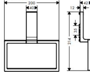
AXOR Universal Rectangular 42623XXX
