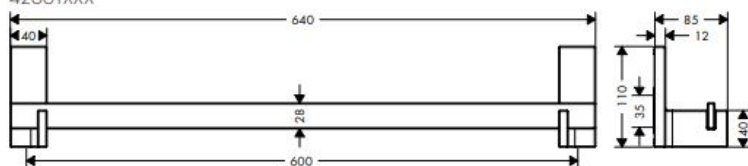
AXOR Universal Rectangular 600 42661XXX
