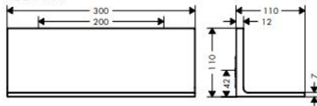
AXOR Universal Rectangular 42644XXX
