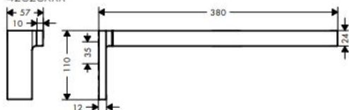
AXOR Universal Rectangular 42626XXX
