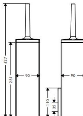
AXOR Universal Rectangular 42655XXX
