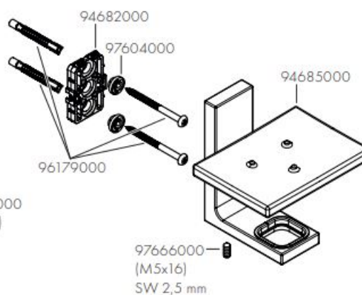
AXOR Universal Rectangular 42605XXX
