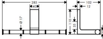
AXOR Universal Rectangular 42657XXX
