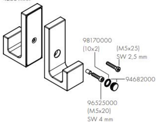
AXOR Universal Rectangular 42639XXX
