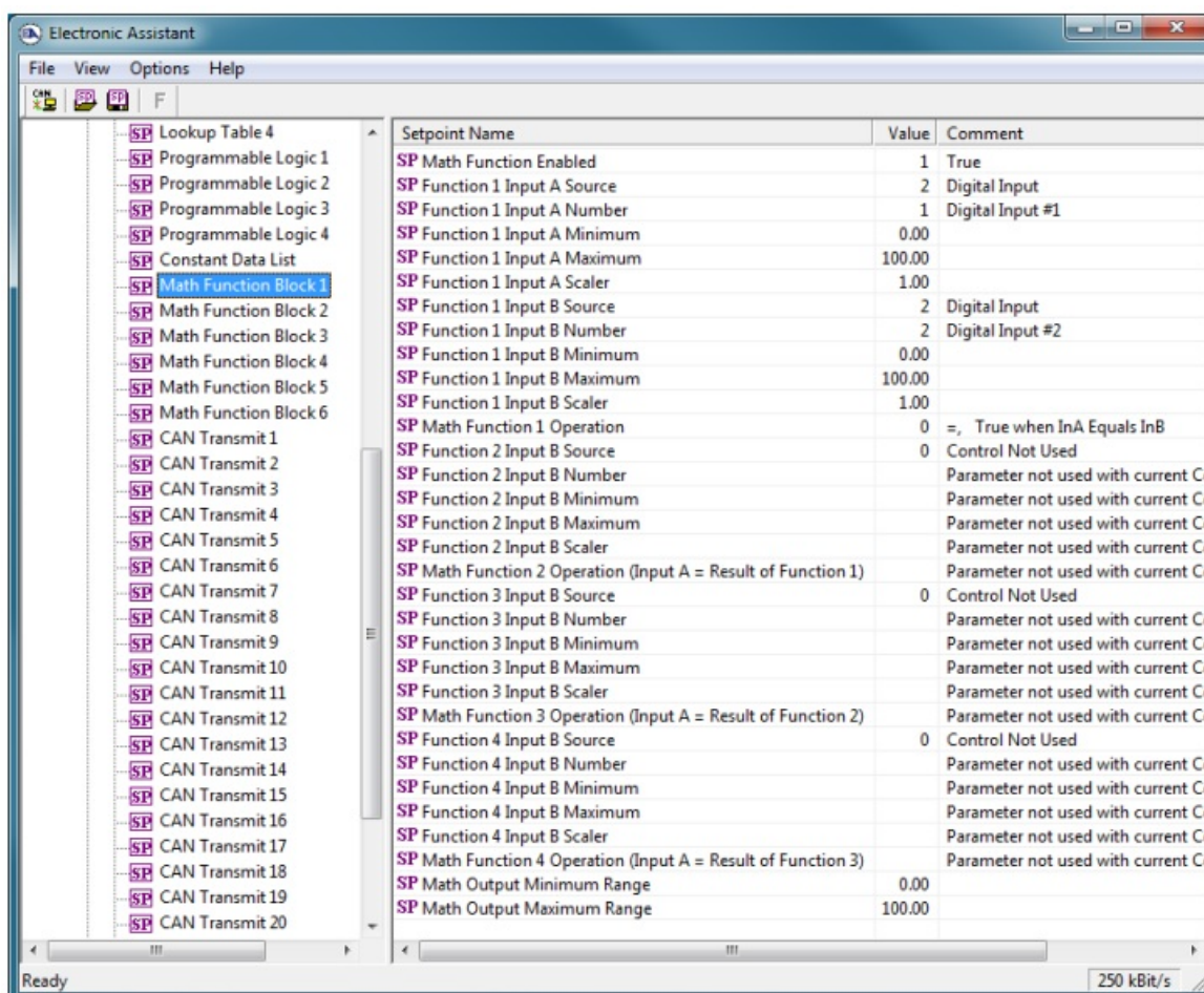
Figure 10 - Screen Capture of Math Function Block Setpoints
