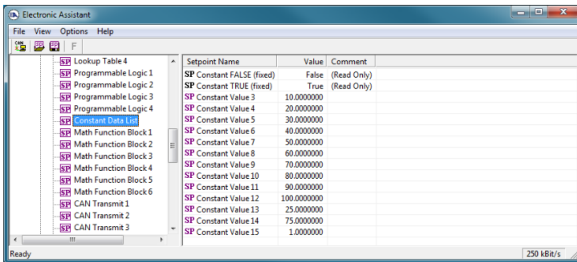
Figure 9 - Screen Capture of Constant Data List Setpoints
