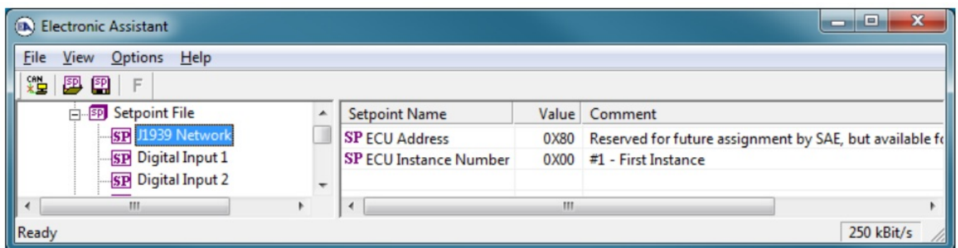
Figure 5 - Screen Capture of J1939 Setpoints
