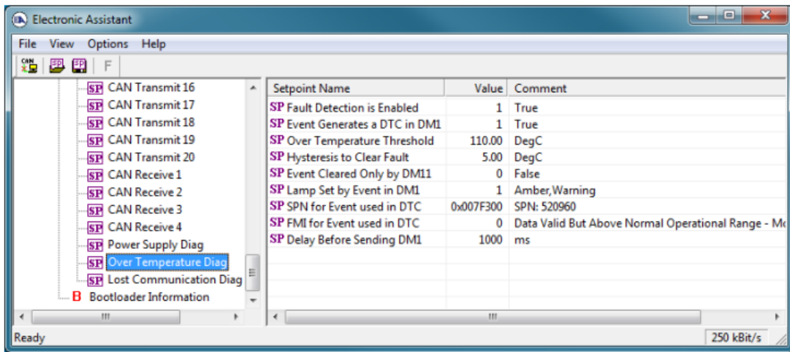
Figure 14 - Screen Capture of Over Temperature Diagnostic Setpoints
