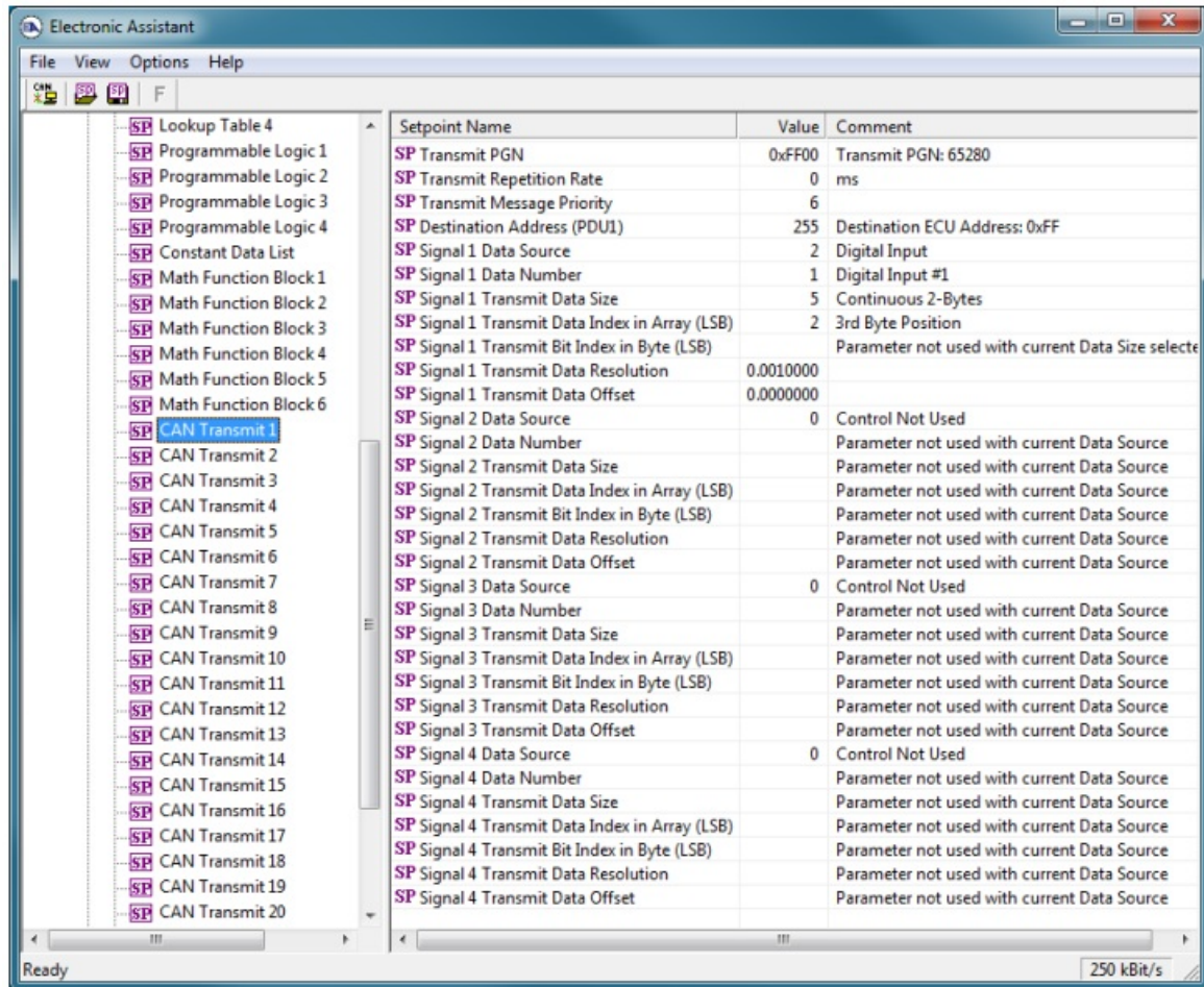
Figure 11 - Screen Capture of CAN Transmit Message Setpoints
