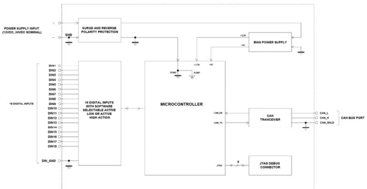
Figure 1 - AX030310 & AX030320 Block Diagram
