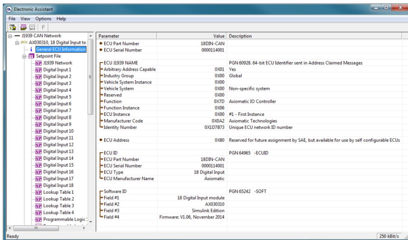
Figure 4 - General ECU Information
