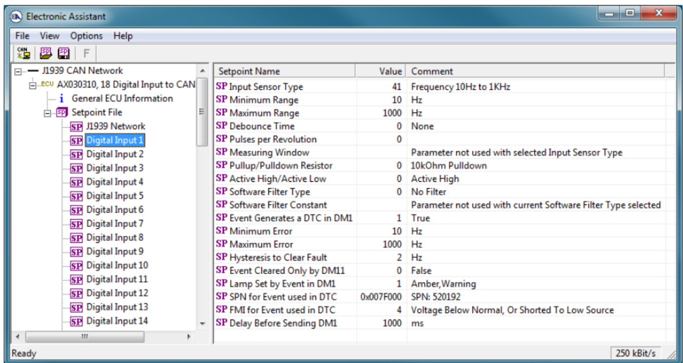
Figure 6 - Screen Capture of Digital Input Setpoints
