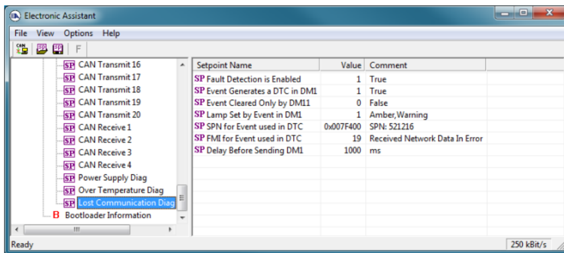
Figure 15 - Screen Capture of Lost Communication Diagnostic Setpoints
