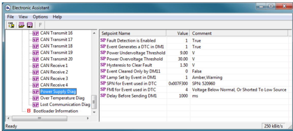
Figure 13 - Screen Capture of Power Supply Diagnostic Setpoints
