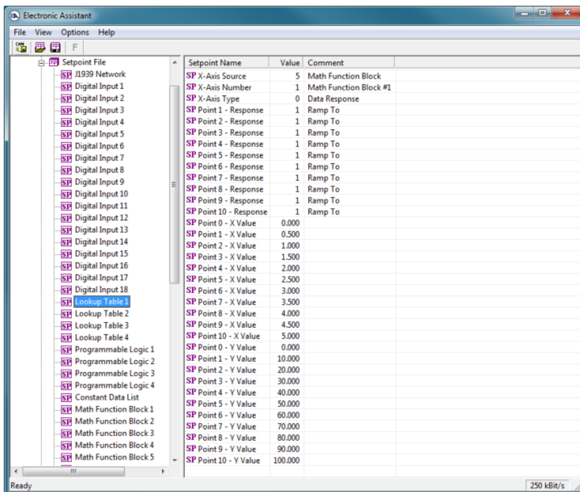
Figure 7 - Screen Capture of Lookup Table Setpoints
