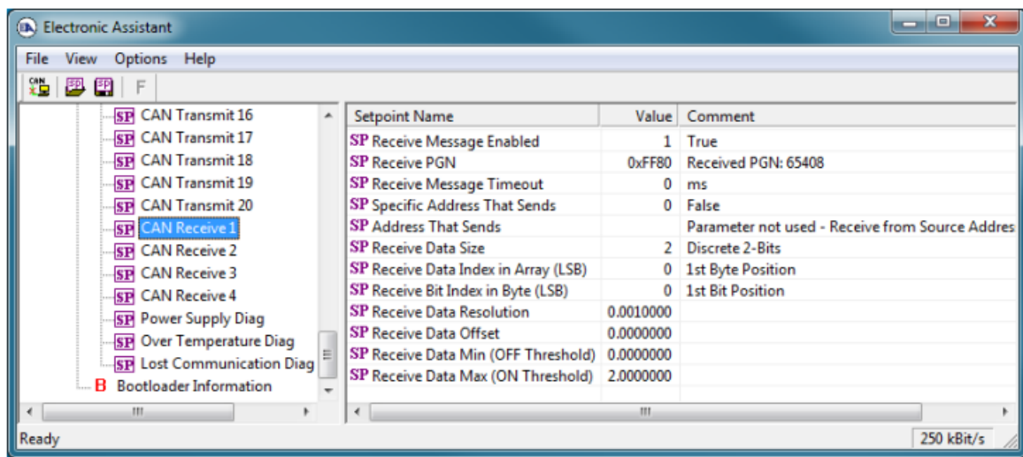
Figure 12 - Screen Capture of CAN Receive Message Setpoints
