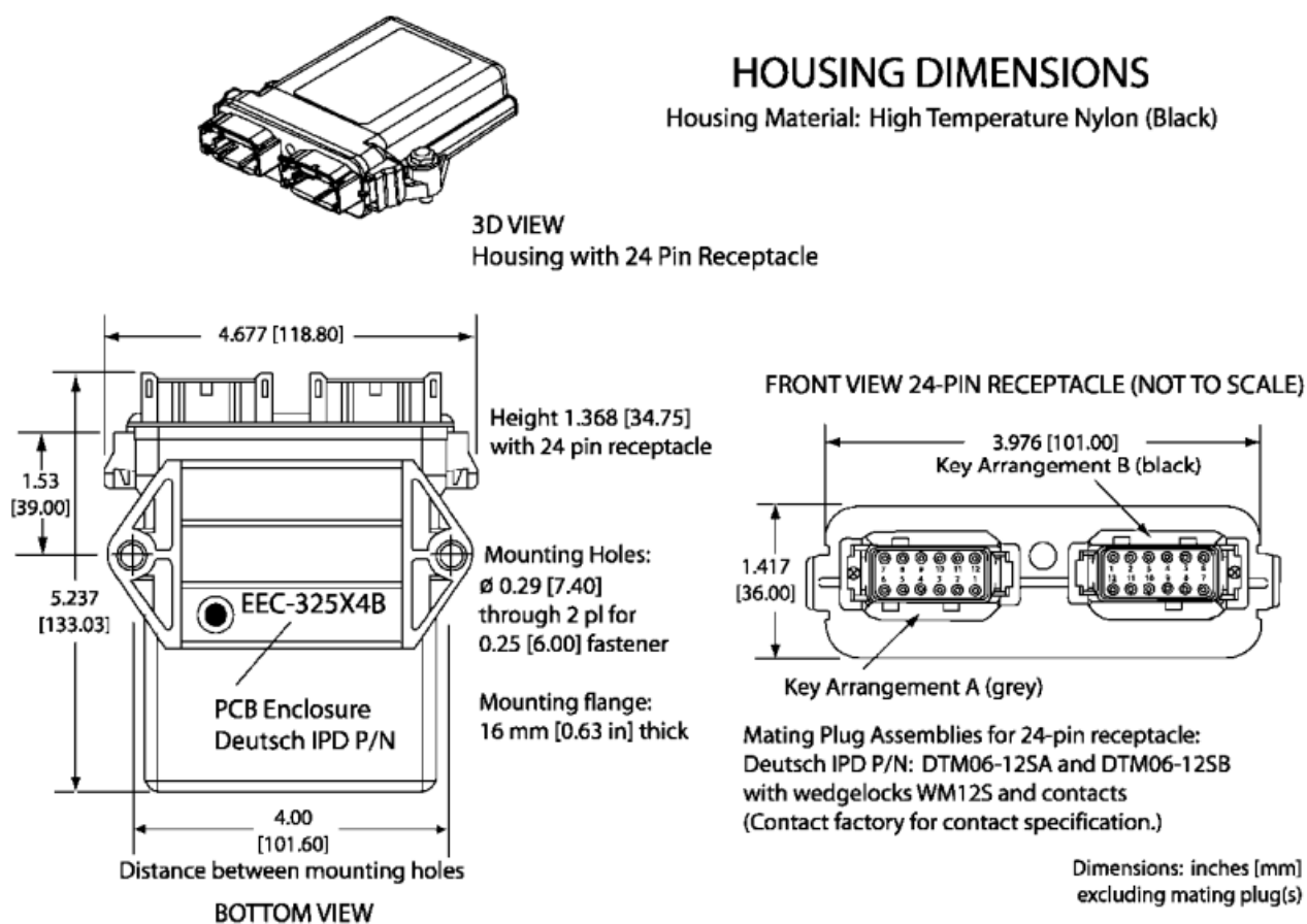
Figure 3 – AX030310 Dimensional Drawing
