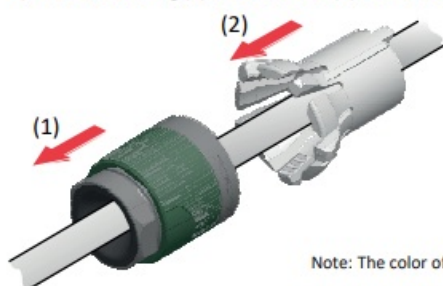
SPEAKON - 2 POLES NL2FXXWS - Ø 6-12mm cables
