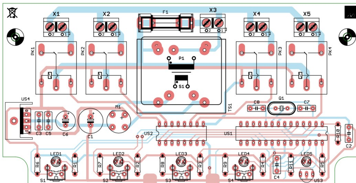
Figure 2. Mounting diagram of a 4-channel switch
