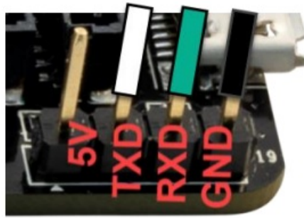
J19 USB-Serial cable to SCIF0 connections
