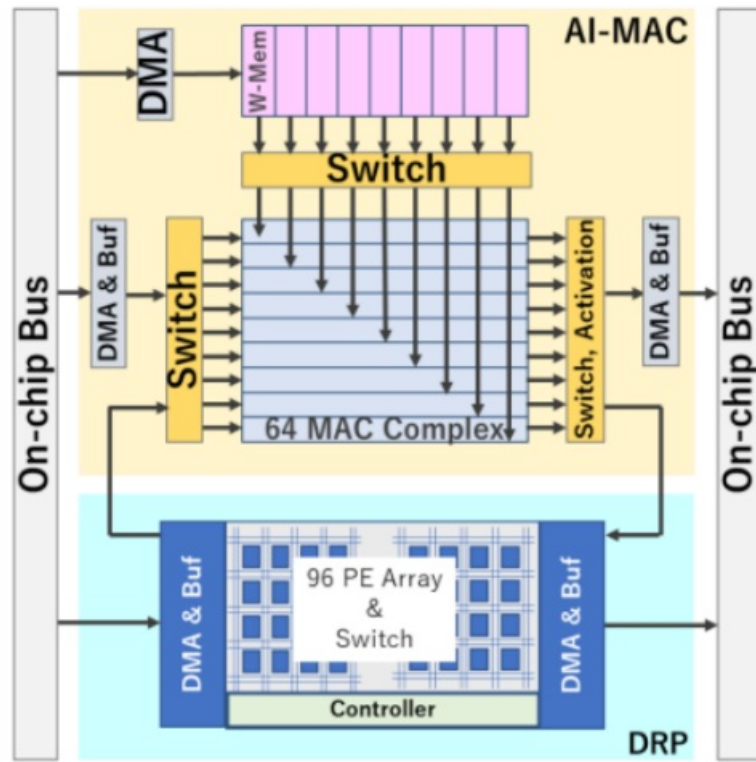
6.4 RZ/V2L Architecture (ACPU bus, MCPU bus, System bus)
