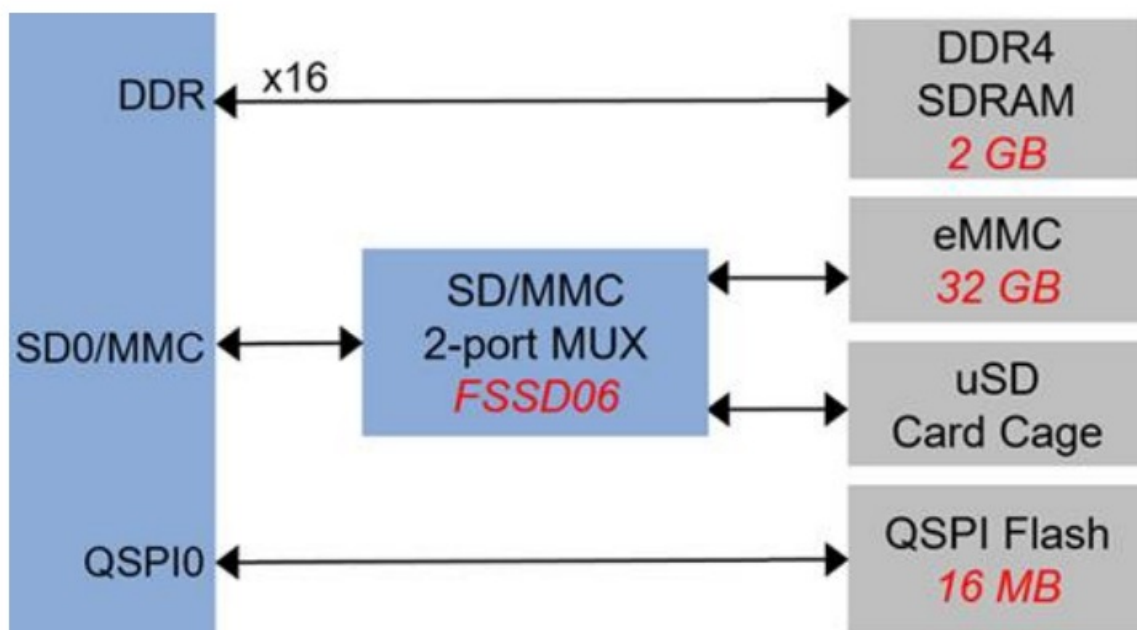
Figure 5 – RZBoard V2L Memory Resources
