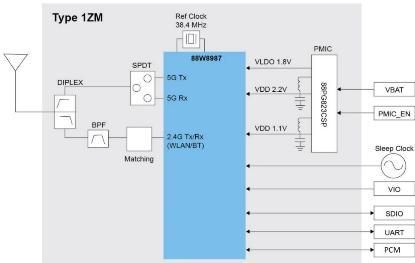
Figure 6 – Murata Type-1ZM Wi-Fi/BT Combo Module Block Diagram
