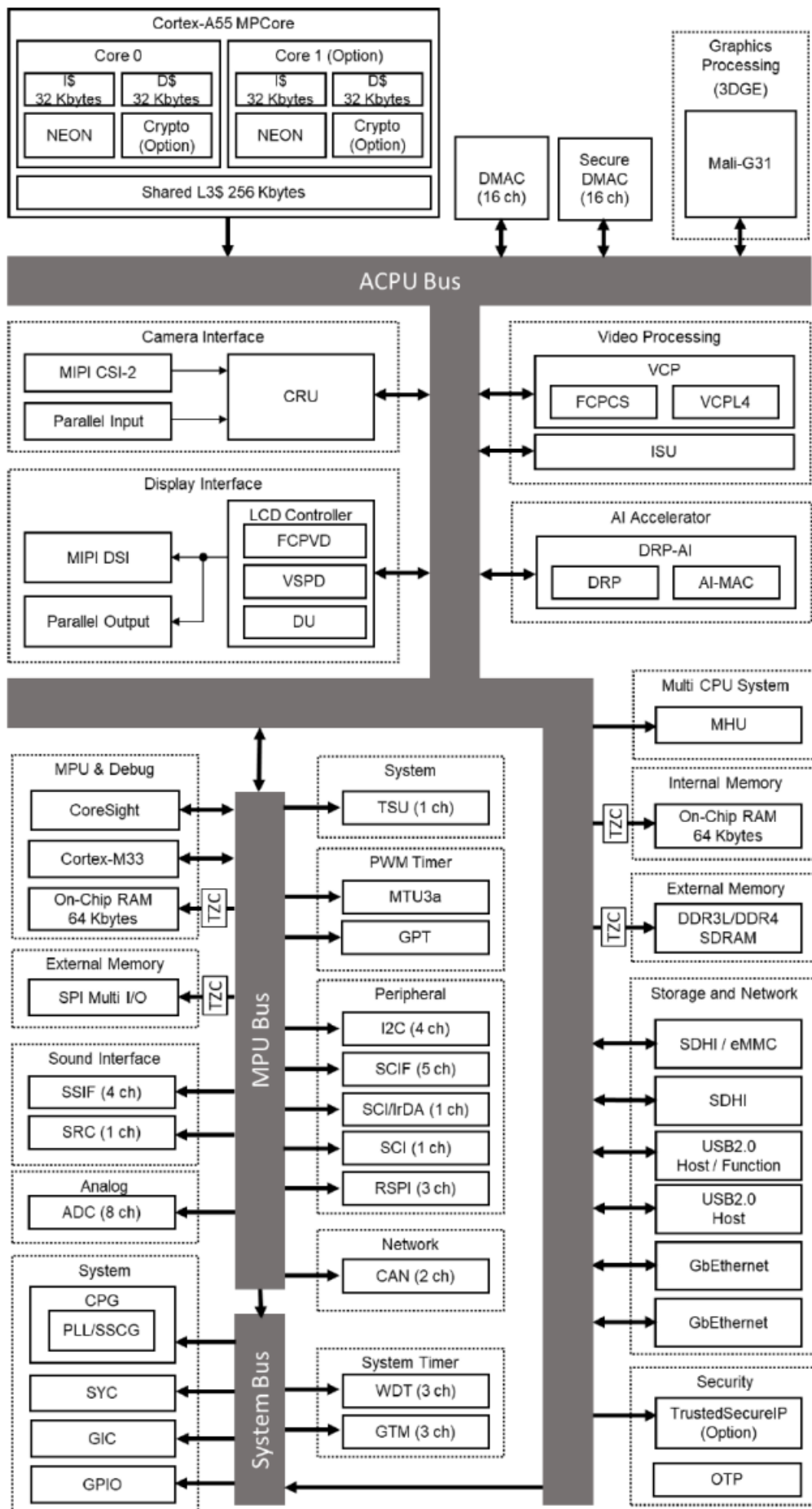
6.5 RZBoard V2L Block Diagram
