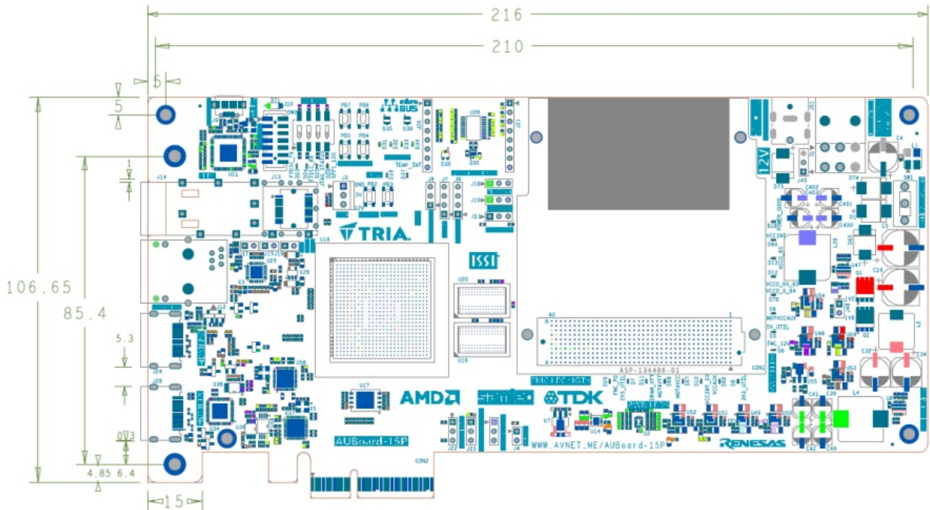
Figure 36 – Mechanical Dimensions
