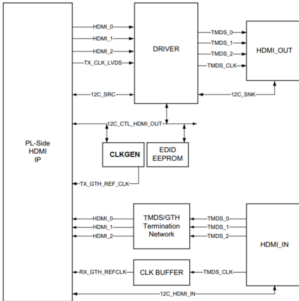
Figure 20 – HDMI Interface Block Diagram
