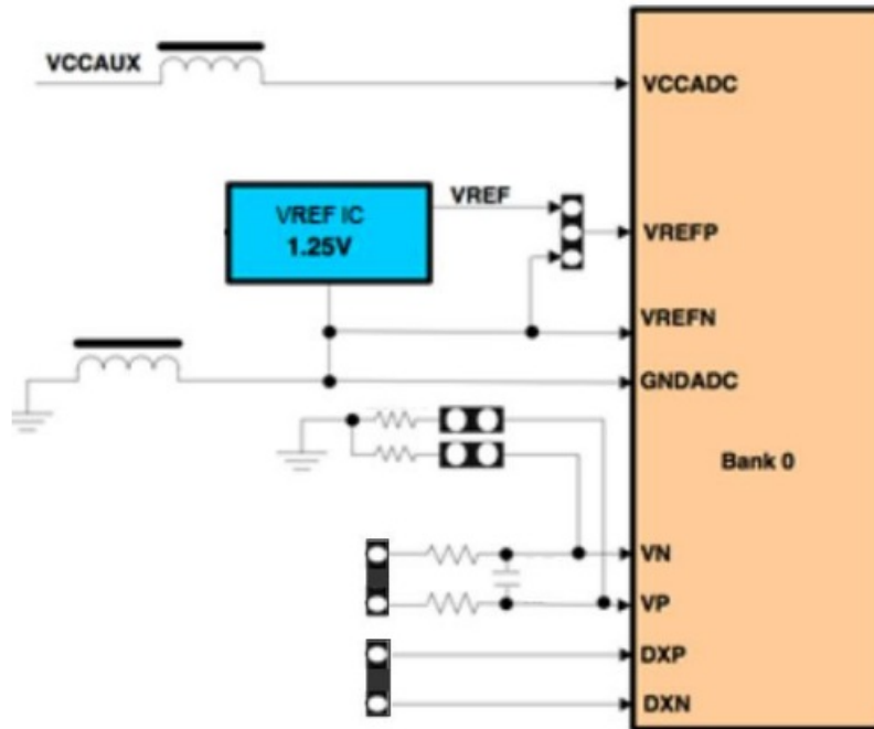
Figure 8 – SYSMON Interface Block Diagram
