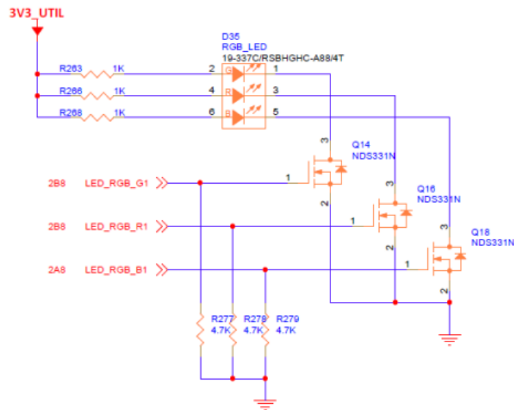
Figure 26 – RGB User LED
