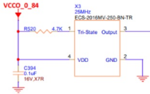
Figure 19 – Ethernet PHY Clock Source
