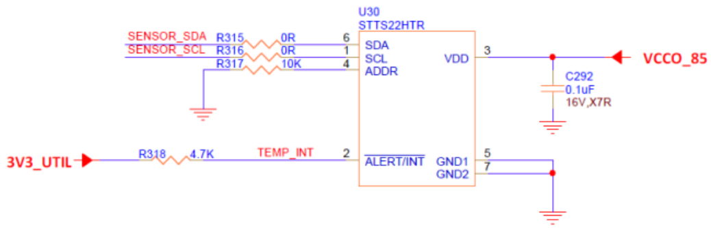
Figure 24 – I2C Temperature Sensor
