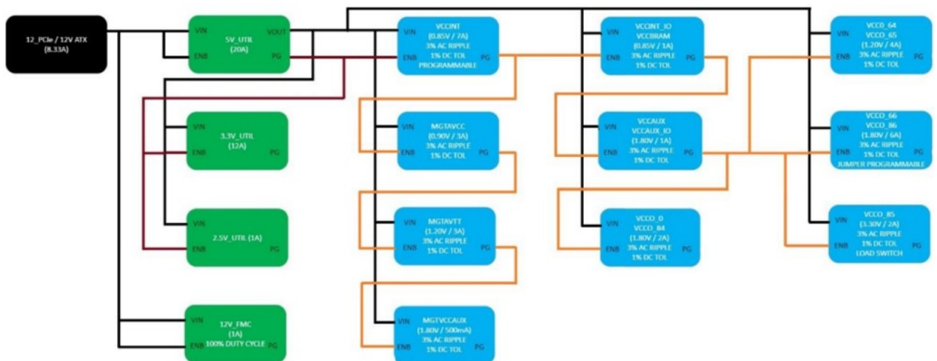
Figure 31 – Power Solution Block Diagram
