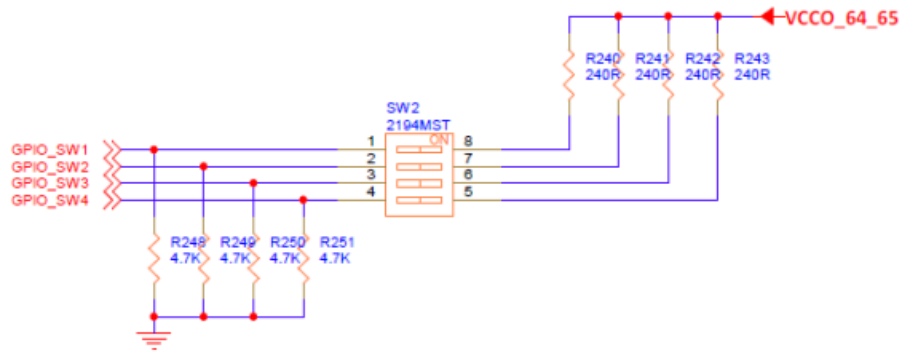
Figure 27 – User Dip Switch
