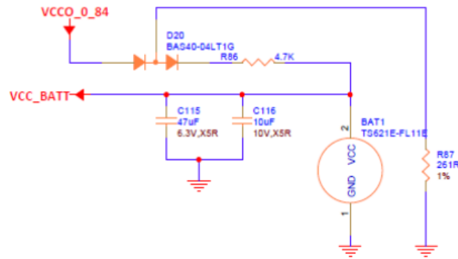
Figure 9 – Battery Backup Circuit
