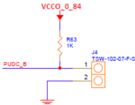
Figure 4 – PUDC_B Header
