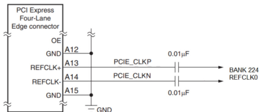
Figure 16 – PCI Express Connector Circuitry
