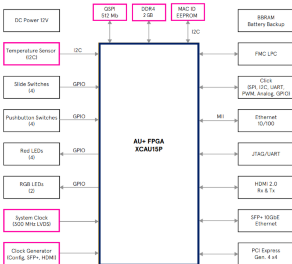
Figure 1 –Development Kit Block Diagram
