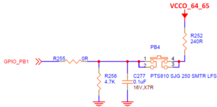
Figure 28 – User Push Buttons
