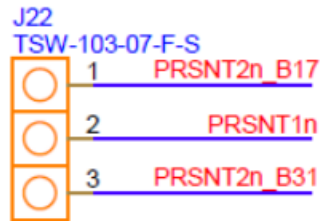
Figure 17 – PCI Express Lane Width Jumper J22
