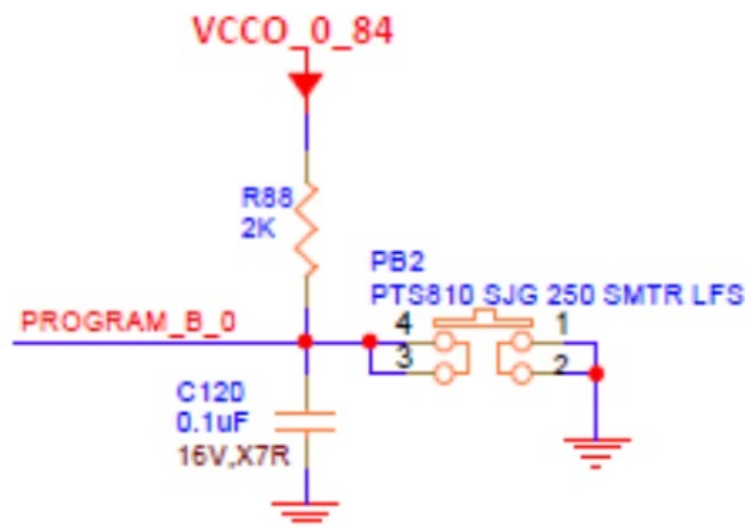
Figure 6 – PROGRAM_B Push Button
