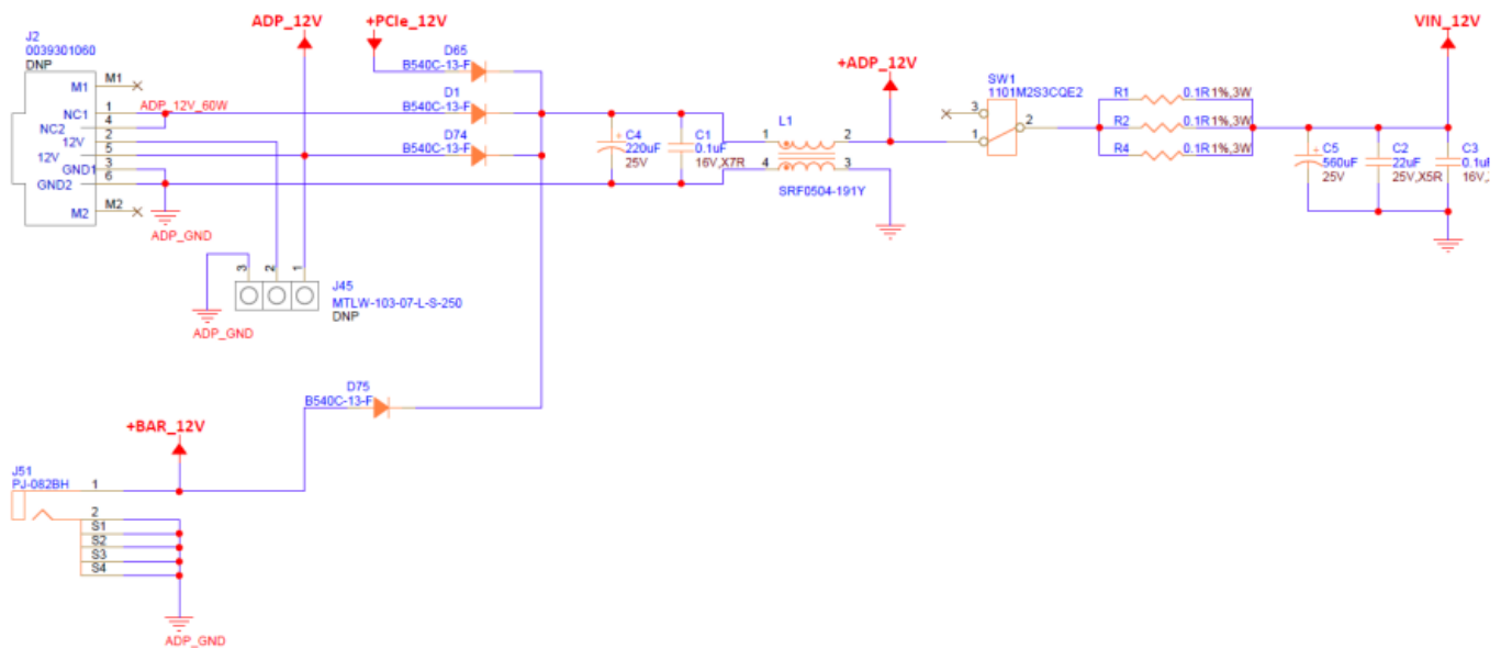
Figure 30 – Power Inputs and On/Off Slide Switch
