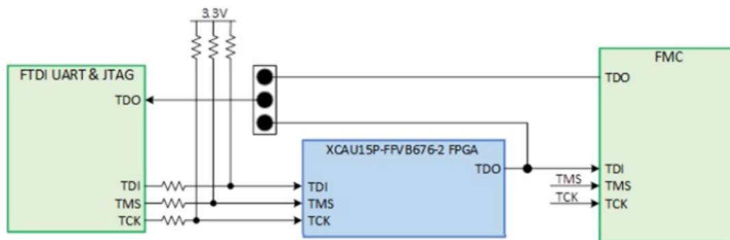
Figure 11 – JTAG Chain Block Diagram
