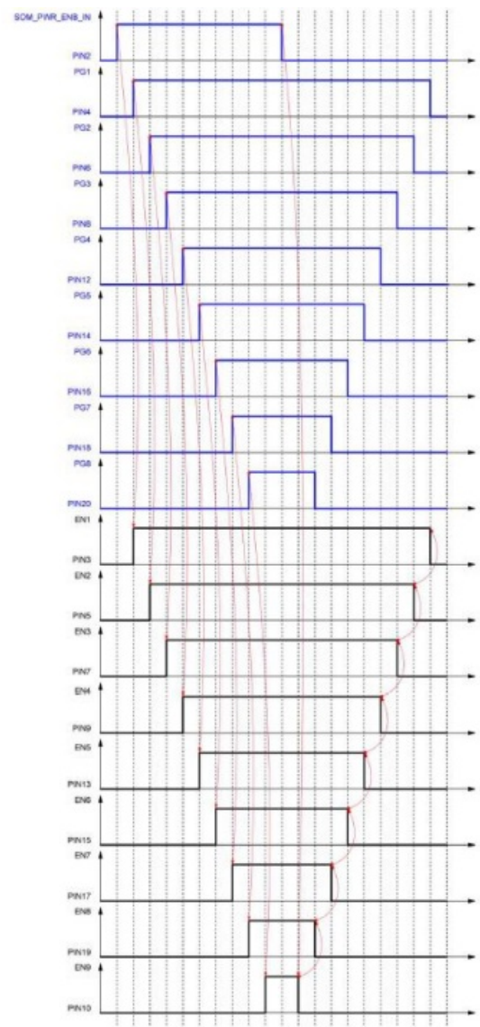
Figure 33 – Power Sequencer Timing Diagram
