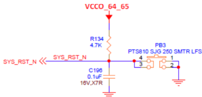
Figure 29 – Reset Push Button
