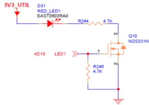
Figure 25 – RED User LED
