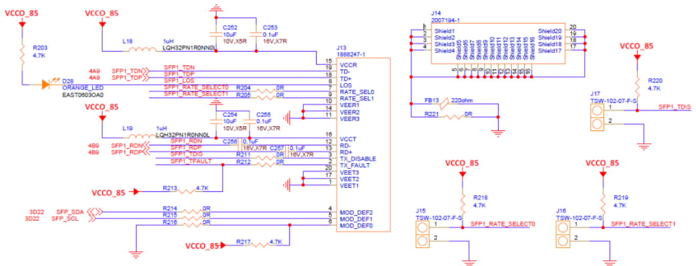
Figure 18 – SFP+ Module Connector Circuitry
