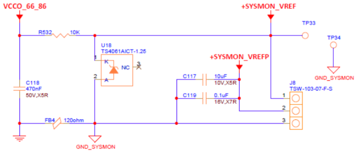
Figure 7 – SYSMON Voltage Reference Select
