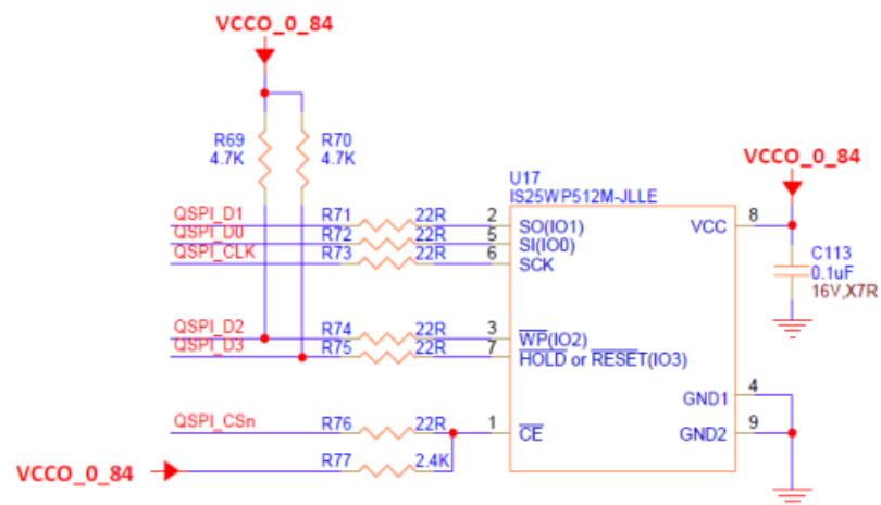
Figure 10 – 512Mb Quad SPI Flash Memory
