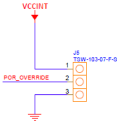
Figure 5 – POR_OVERRIDE Header
