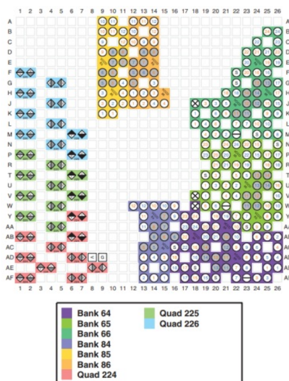
Figure 2 – FFVB676 Package Diagram
