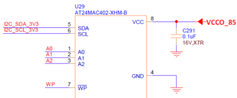
Figure 23 – MAC ID EEPROM
