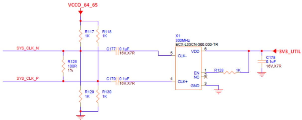
Figure 12 – System Clock Source
