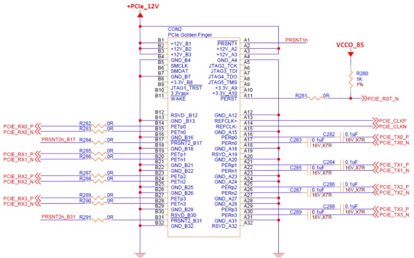
Figure 15 – PCI Express Clock Source
