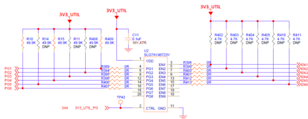
Figure 34 – Power Sequencer Schematic
