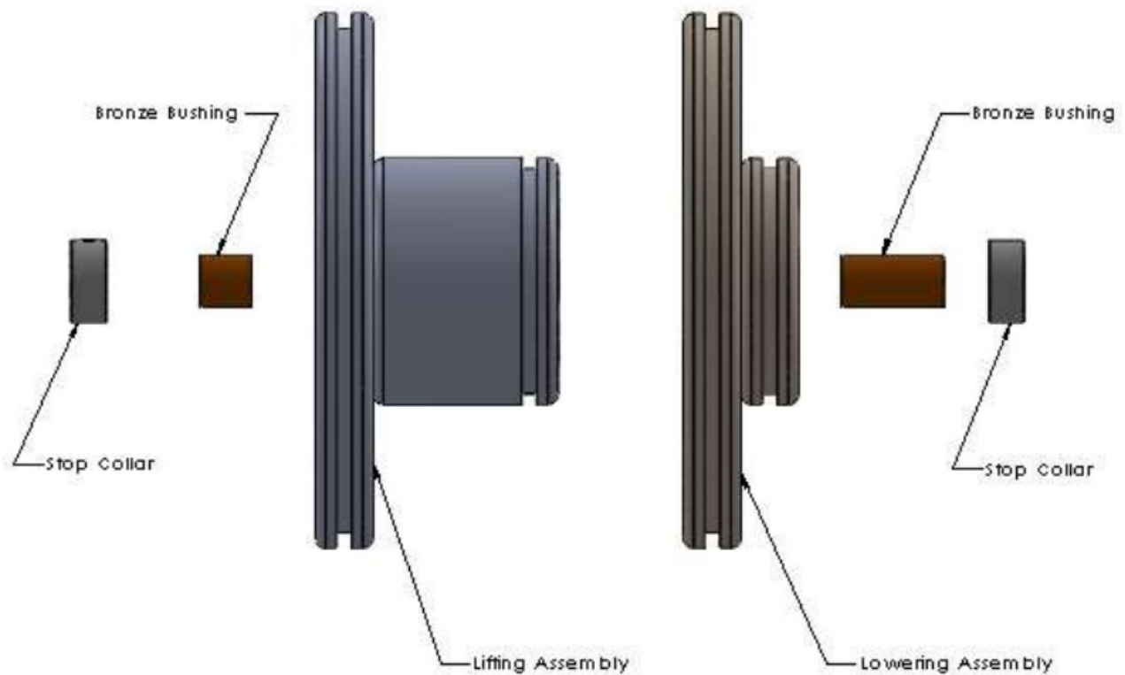
Fig. 3-P – Cam-cylinders Configuration for PDL (right side view)
