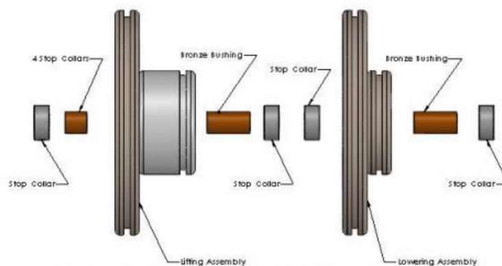
Fig. 3-V – Cam-cylinders Configuration for V-Series (right side view)
