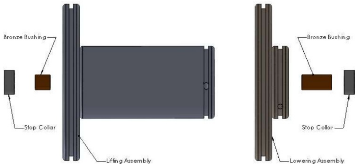
Fig. 3-T – Cam-cylinders Configuration for TDL (right side view)
