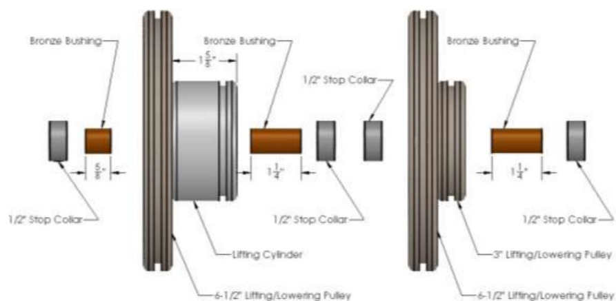
Fig. 3-V – Cam-cylinders Configuration for V-Series (right side view)
