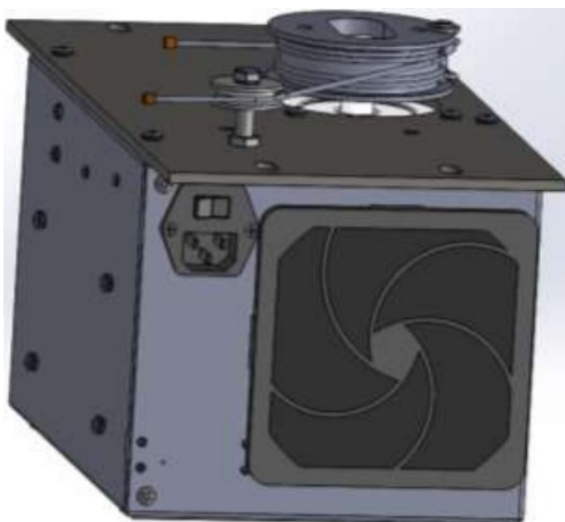
Fig. 2b – E-Lift Cable Routing (rear view)
