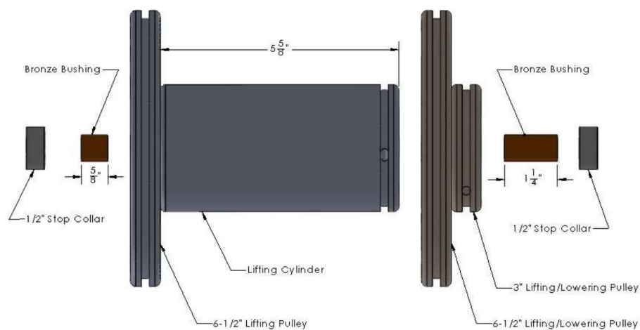
Fig. 3-S – Cam-cylinders Configuration for SDL (right side view)
