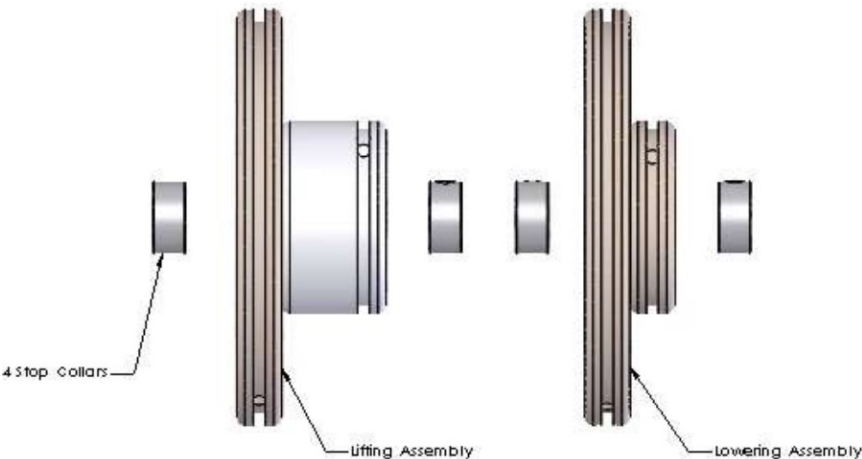
Fig. 3-A/N – Cam-cylinders Configuration for A-Series with Negative Dobby (right side)
