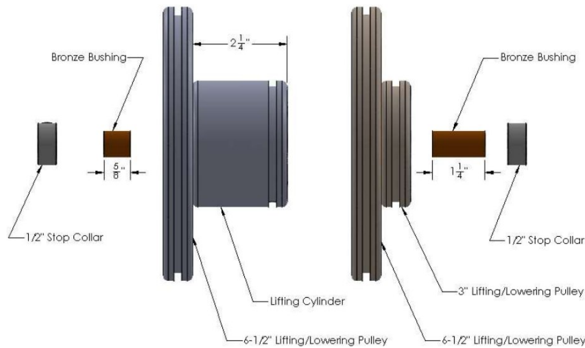
Fig. 3-P – Cam-cylinders Configuration for PDL (right side view)
