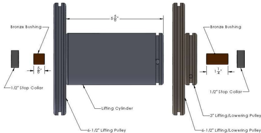
Fig. 3-T – Cam-cylinders Configuration for TDL (right side view)
