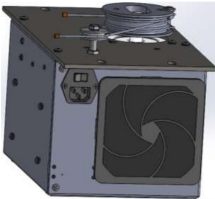
Fig. 2b – E-Lift Cable Routing (rear view)
