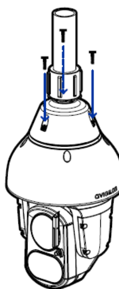
Figure 6: Securing the camera to the NPT adapter.
