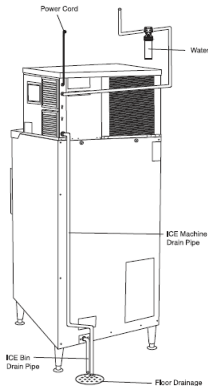
Back View of 194HBN18030 Installation
