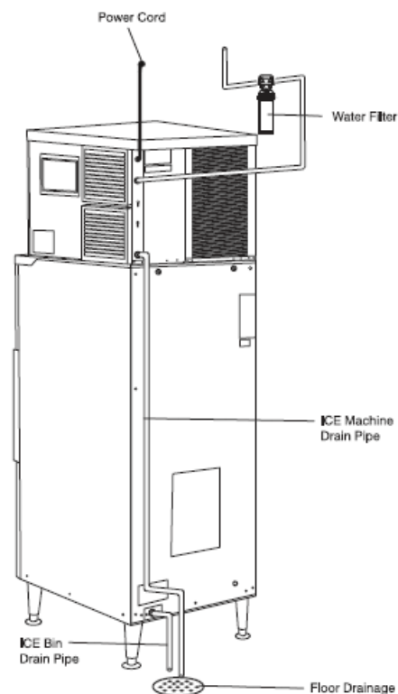
Back View of 194HBN12022 Installation
