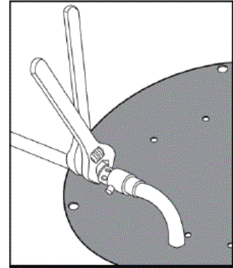
REMOVAL OF THE ORIFICE ASSEMBLY
