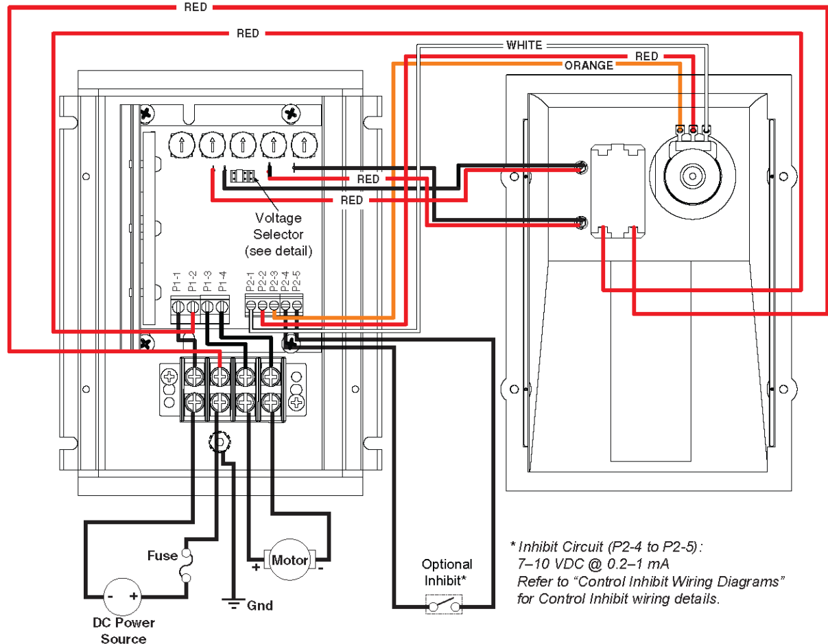
GSD1-48-10N4X BASIC WIRING DIAGRAM
