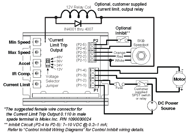
GSD1-48-xxC BASIC WIRING DIAGRAM
