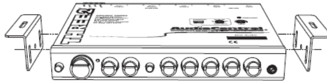
Figure 3: THREE.2 with mounting brackets
