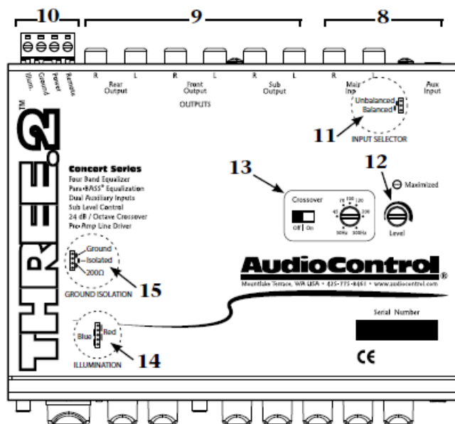
Figure 3: Top View of THREE.2, with a peek at what's inside
