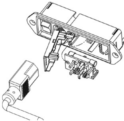
Figure 3. Power entry module door and fuse block.
