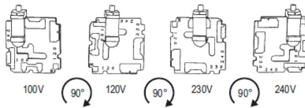
Figure 5. Voltage card selector orientation.
