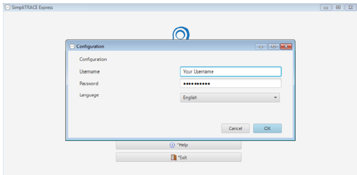
Figure 1: Access Page
