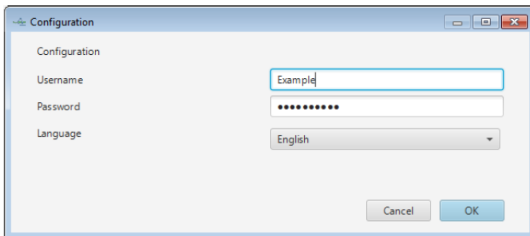
Figure 15: Login settings
