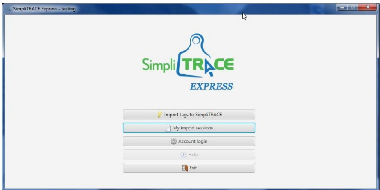
Figure 3: Homepage
