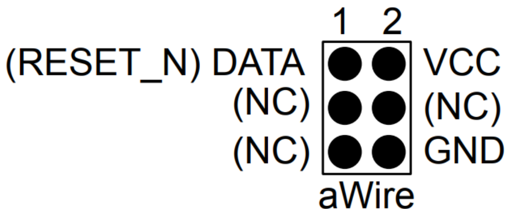
Figure 4-8. aWire Header Pinout
