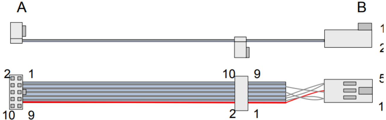
Figure 3-2. Debug Cable Pinout
