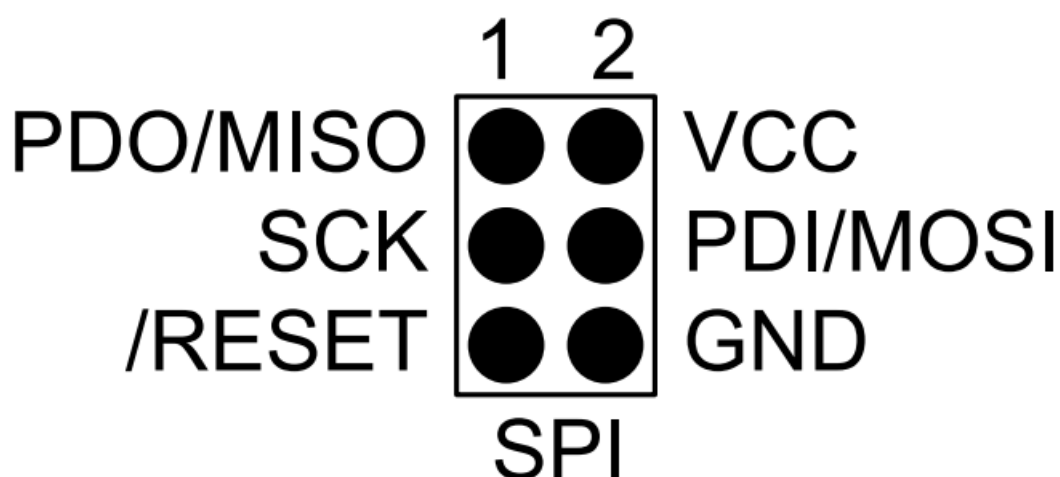
Figure 4-10. SPI Header Pinout
