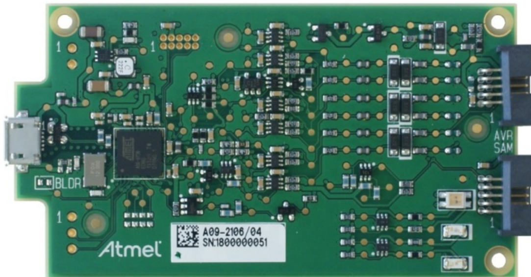
Figure 2-3. Atmel-ICE PCBA Kit Contents
