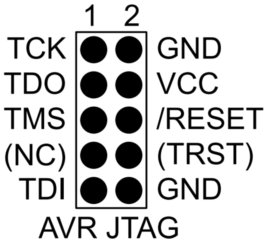
Figure 4-6. AVR JTAG Header Pinout
