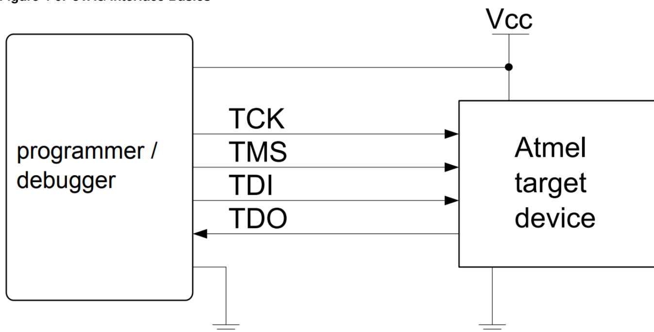
Figure 4-9. JTAG Interface Basics
