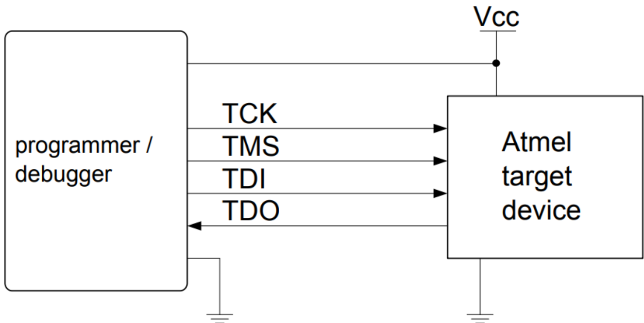
Figure 4-1. JTAG Interface Basics
