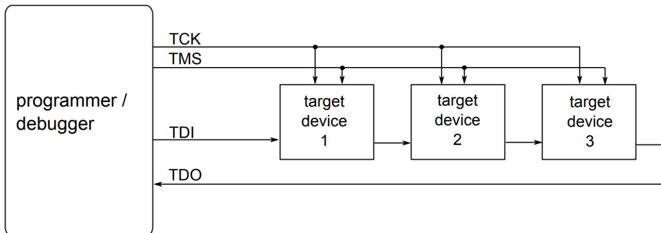
Figure 4-7. JTAG Daisy Chain
