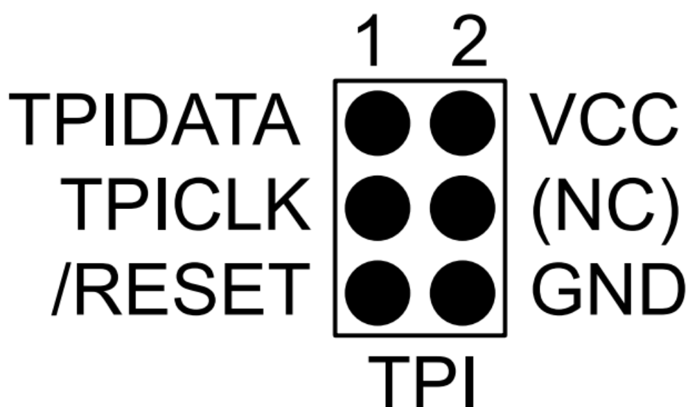
Figure 4-13. TPI Header Pinout
