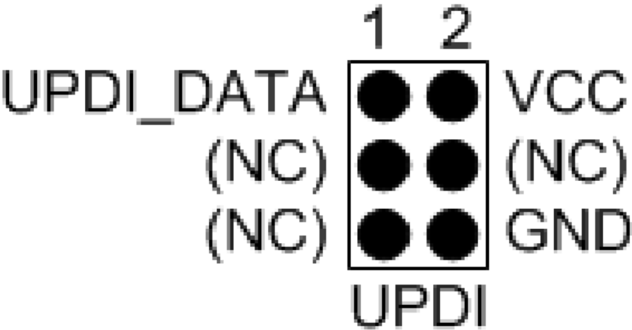
Figure 4-12. UPDI Header Pinout
