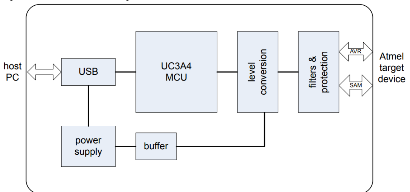
Figure 5-1. Atmel-ICE Block Diagram
