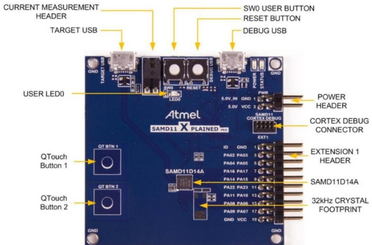
Figure 1-1. SAM D11 Xplained Pro Evaluation Kit Overview
