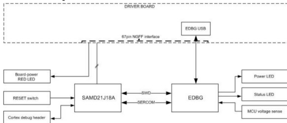
Figure 5-2. MCU Board Block Diagram
