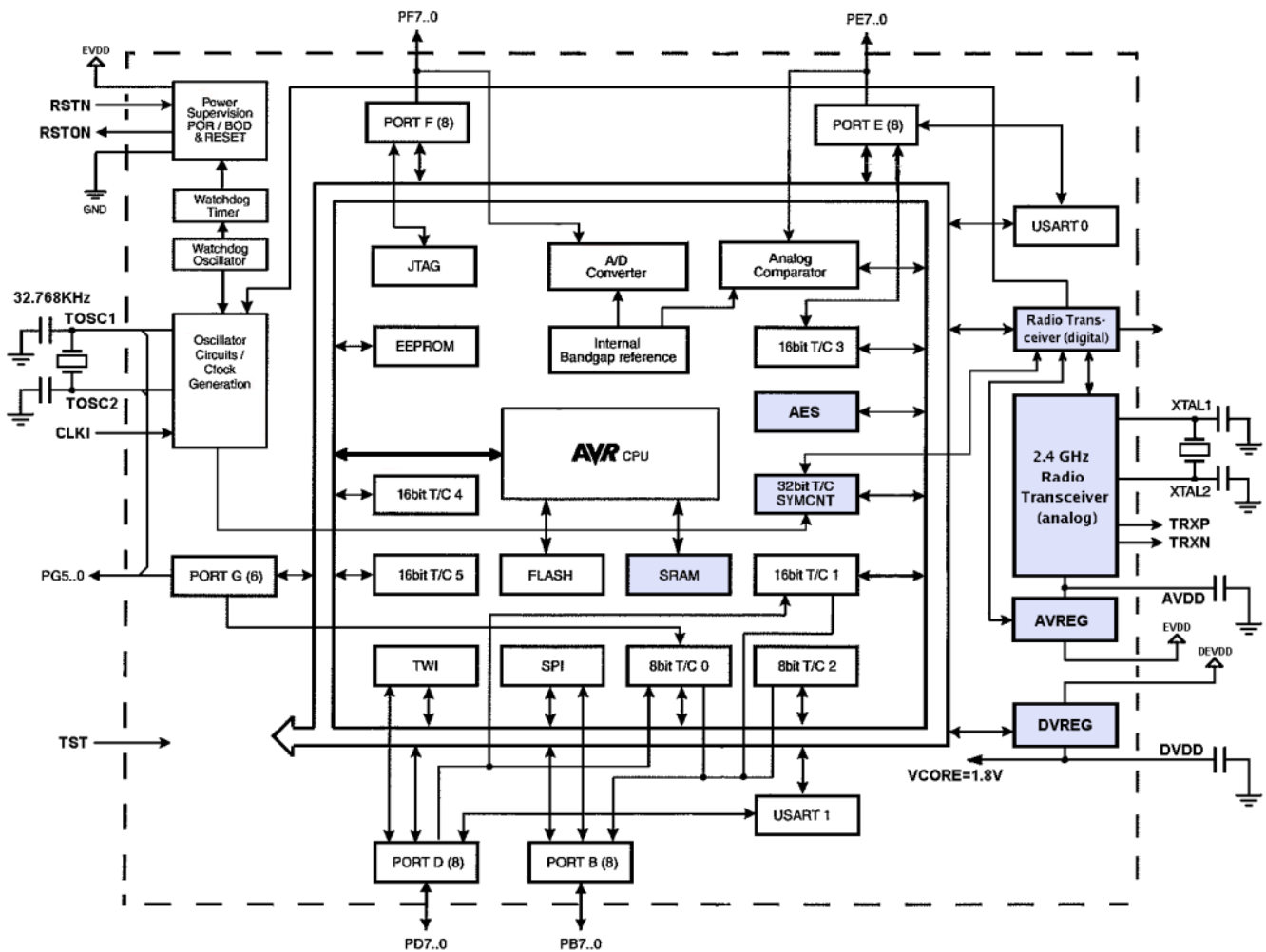
Figure 3-1 Block Diagram
