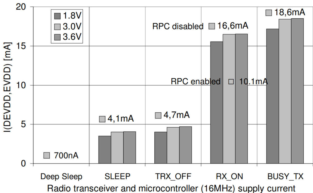
Figure 3-2 Radio transceiver and microcontroller (16MHz) supply current
