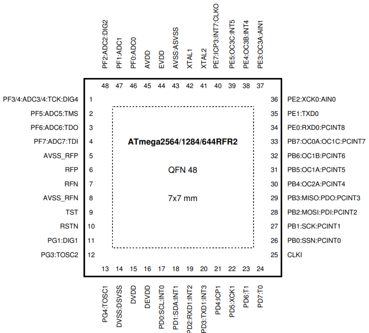
Figure 1-1. Pinout ATmega2564/1284/644RFR2
