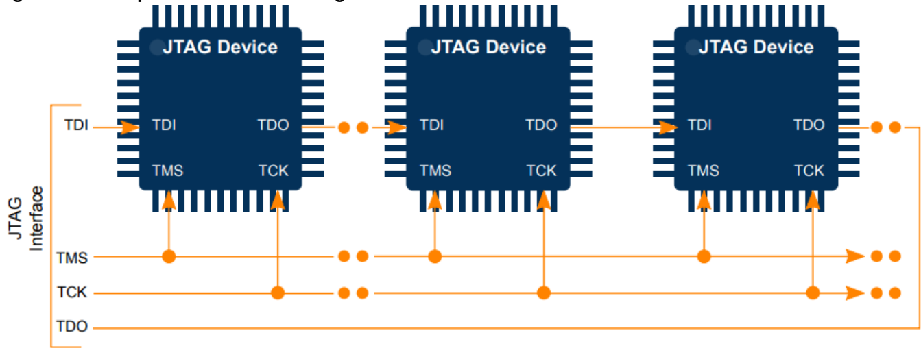
Figure 2-2 Multiple Device JTAG Configuration
