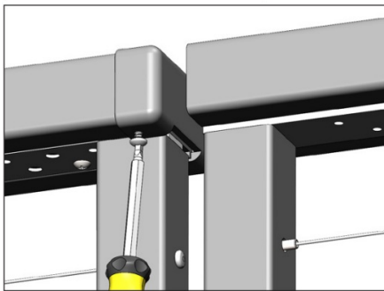
NOTCHED END CAPS
