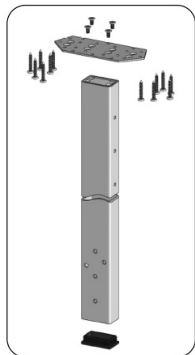
R. Fascia Mount 42" End/Corner Post Kit (S0904-*XX42-EC)
