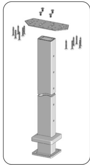
O. Surface Mount 42" End/Corner Post Kit (S0905-*XX42-EC)
