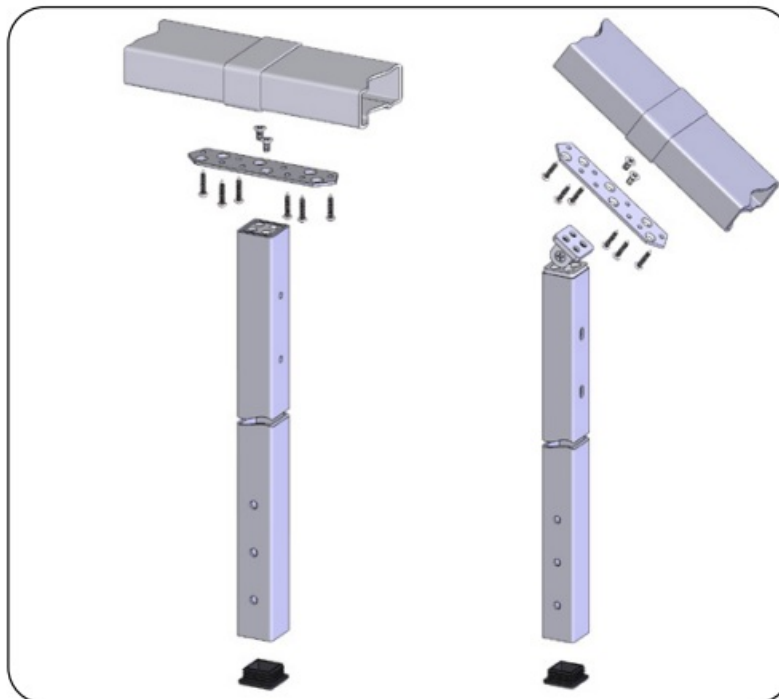
P. Fascia Mount Post Kit 36" (S0904-*XX36) 42" (S0904-*XX42)
