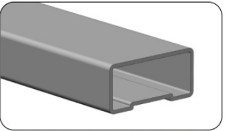
H. Top Rail - 4 ft. (S0904-AR48-*XX) Top Rail - 6 ft. (S0904-AR72-*XX) Top Rail - 8 ft. (S0904-AR96-*XX)
