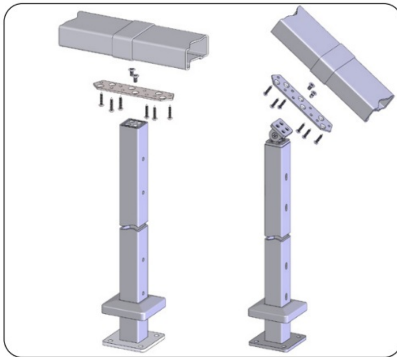
M. Surface Mount Post Kit 36" (S0905-*XX36) 42" (S0905-*XX42)
