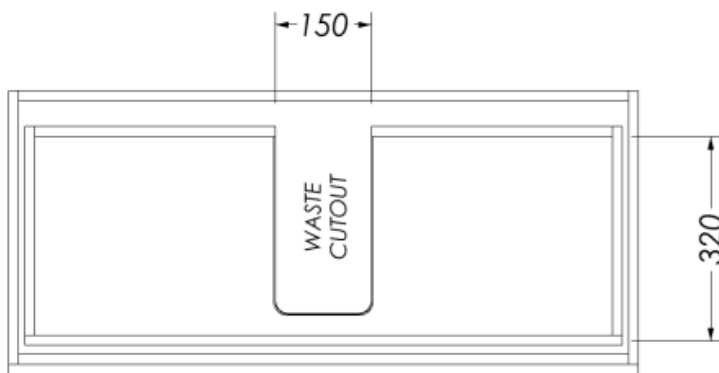
COSMETICS DRAWER (OPTIONAL) CROSS SECTION
