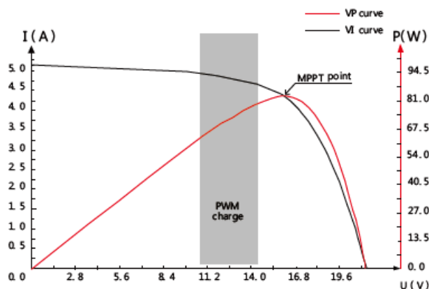
Fig.1-2 Output Characteristic Curve for Solar Battery
