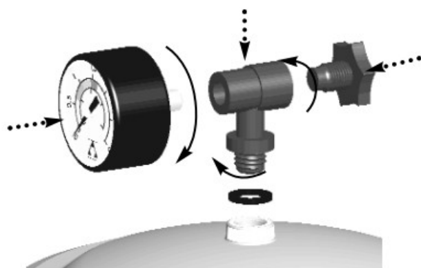
Assembly of the manometer (with lateral valve)
