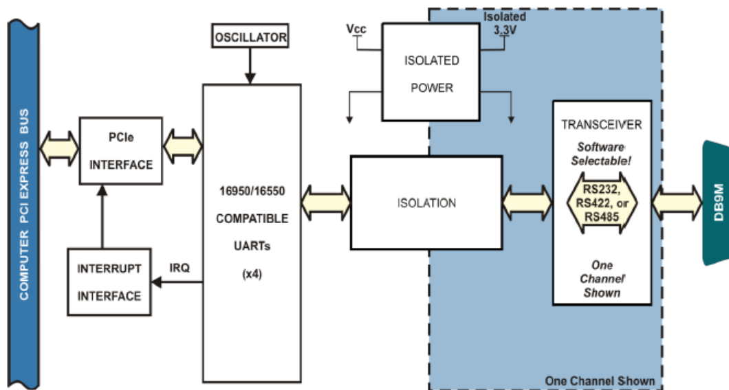
Figure 1-1: Block Diagram
