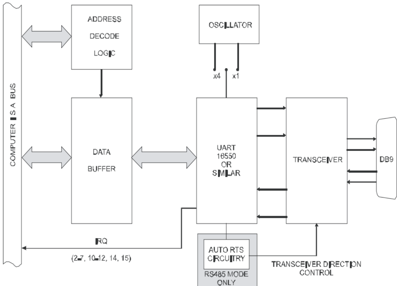
Figure 1-1: Block Diagram(Only one serial channel shown)
