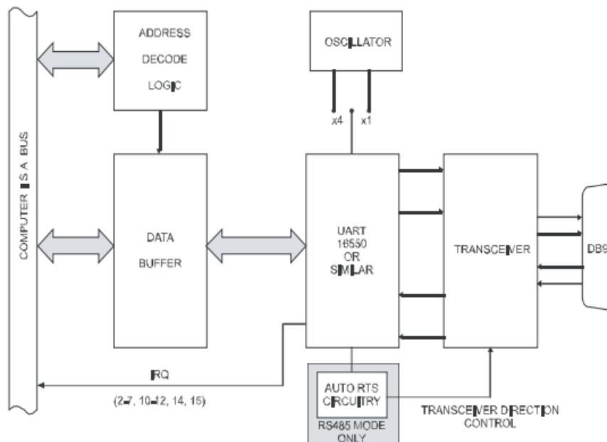
Figure 1-1: Block Diagram(Only one serial channel shown)
