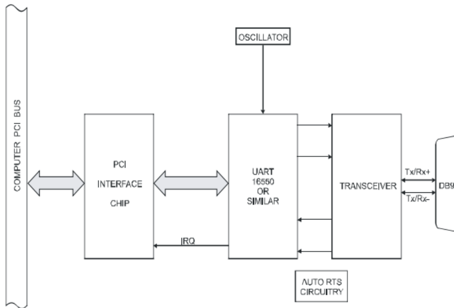
Figure 1-1: Block Diagram(Only one serial channel shown)
