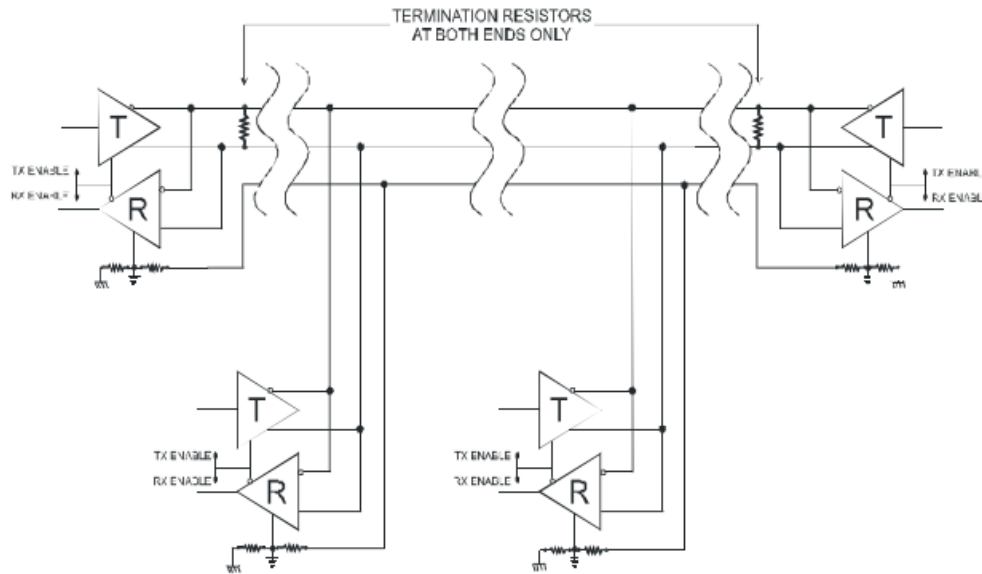
Figure A-1: Typical RS485 Two-Wire Multidrop Network
