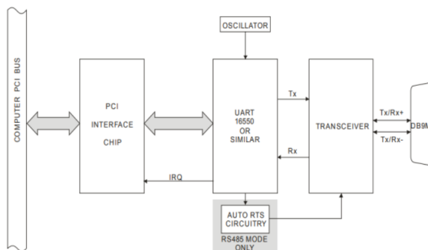
Figure 1-1: Block Diagram
