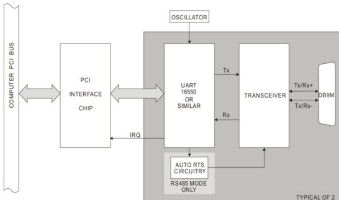
Figure 1-1: Block Diagram
