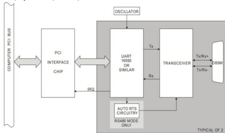
Figure 1-1: Block Diagram
