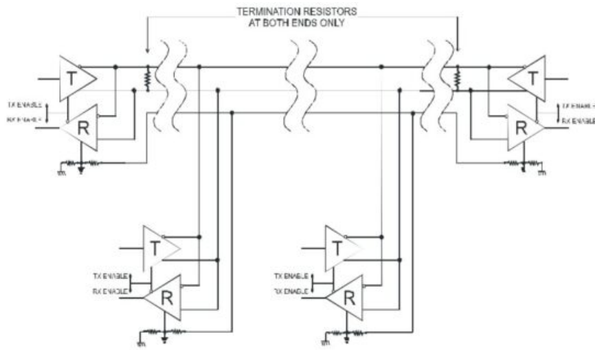
Figure A-1: Typical RS485 Two-Wire Multidrop Network
