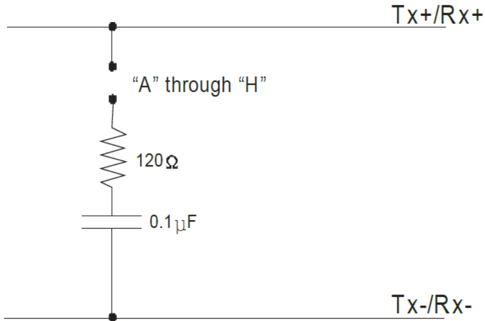
Figure 3-1: Simplified Termination Schematic
