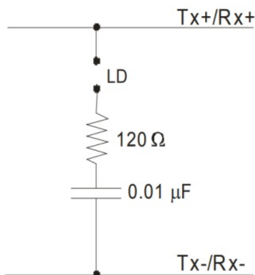
Figure 3-1: Simplified Termination Schematic
