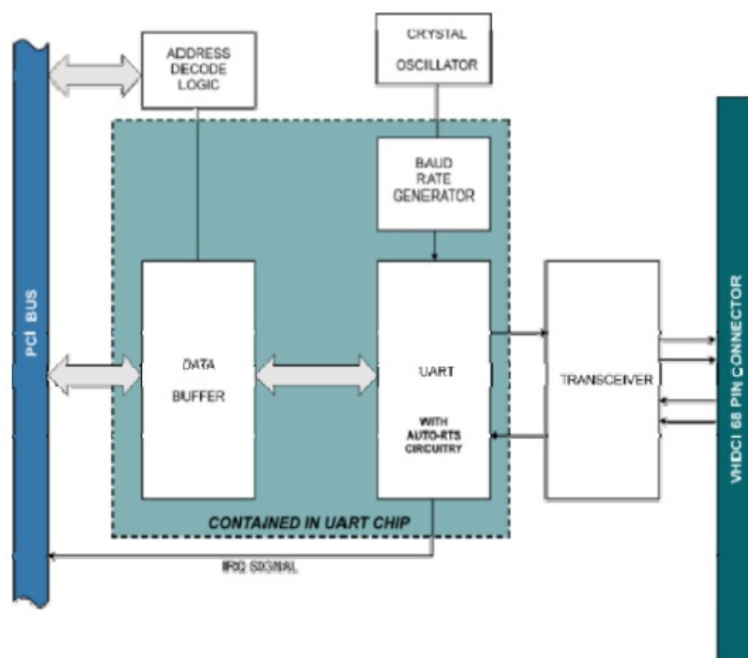
Figure 1-1: Block Diagram (Only one serial channel shown)
