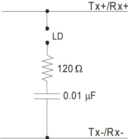
Figure 3-1: Simplified Termination Schematic
