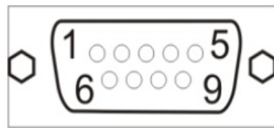
Figure 6-1: DB9 Male Connector Pin Locations
