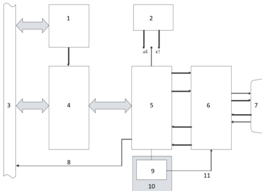
Figure 1-1: Block Diagram(Only one serial channel shown)
