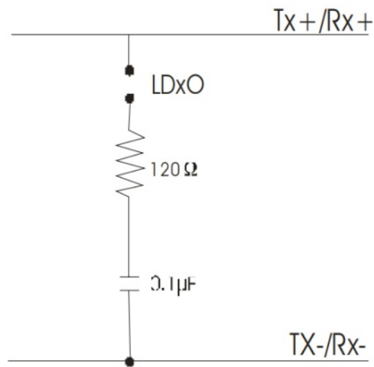
Figure 3-1: Simplified Termination Schematic
