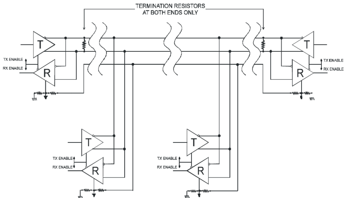
Figure A-1: Typical RS485 Two-Wire Multidrop Network
