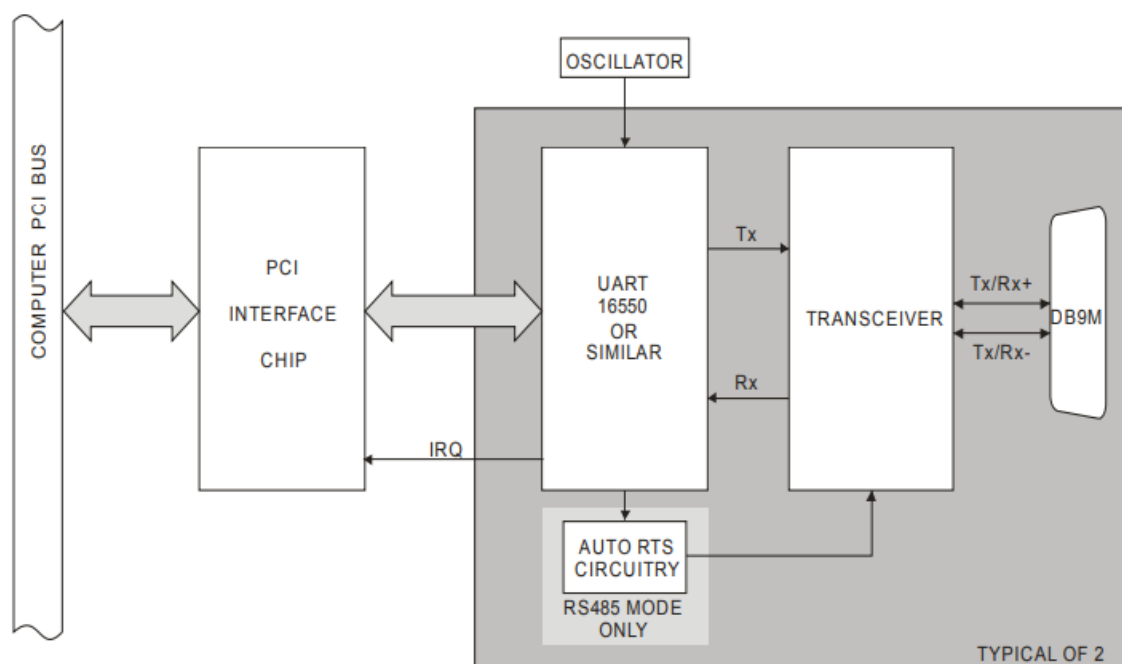
Figure 1-1: Block Diagram
