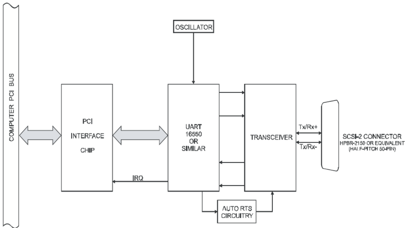
Figure 1-1: Block Diagram (only one serial channel shown)
