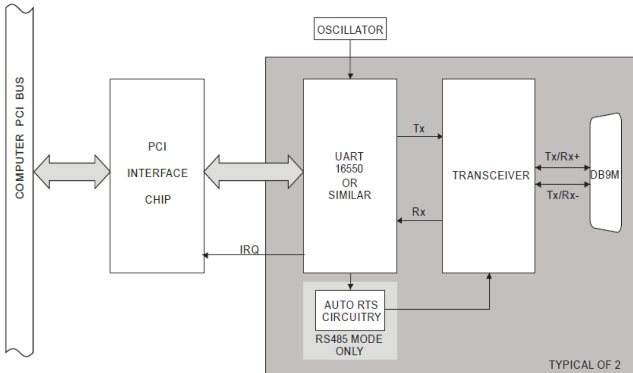
Figure 1-1: Block Diagram
