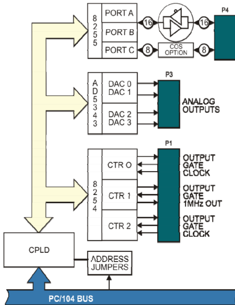
Figure 1-3: 104-AO12-4 Analog Output Board Block Diagram
