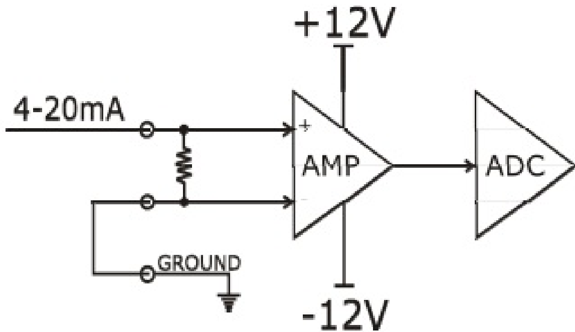
Figure 5-3: 4-20mA Source to Differential Input
