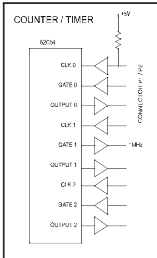
Figure 5-6: Counter Timer Block Diagram
