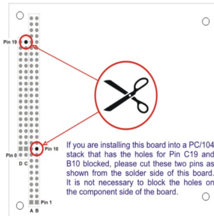
Figure 2-1: PC/104 Key Information
