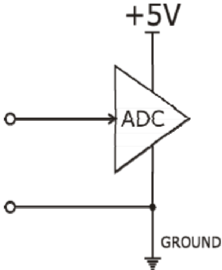
Figure 5-4: Single-Ended Input Stage
