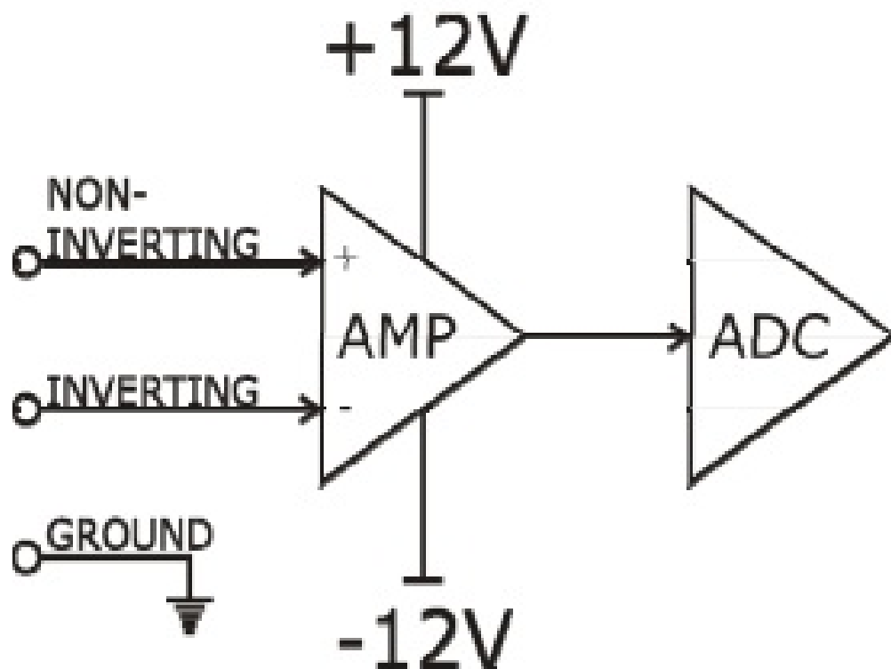
Figure 5-1: Differential Source to Differential Input
