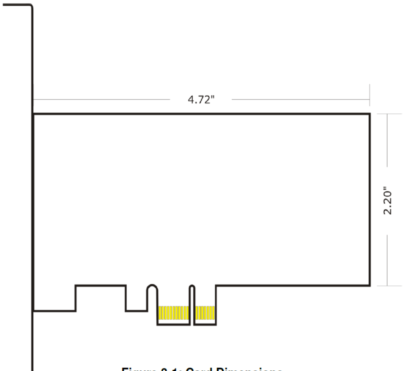
Figure 3-1: Card Dimensions
